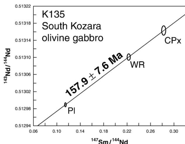
Fig. 9. Sm–Nd-isochron plot of an olivine-bearing cumulate gabbro from South Kozara. The three data points (PI=Plagioclase, WR=whole-rock, CPx=clinopyroxene) fit onto an isochron with an age of 158 \pm 8 Ma (MSWD 0.0109). The initial ^{143}\text{Nd}/^{144}\text{Nd} value is 0.512871 \pm 9 (see Table 2). See Figs. 4 and 12 for sample locality.
