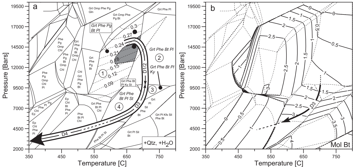
Fig. 13. Equilibrium phase diagrams for the measured bulk rock chemistry of the CM metapelitic sample LK13 taken from the outcrop depicted in Figure 4 (compare micrographs given in Figure 12a–c). The diagrams are calculated with the program DOMINO (De Capitani 1994) and they postulate distinct stable phase assemblages and corresponding mineral composition based on thermodynamic properties defined in the database (JUN92). Bulk rock chemistry is determined by powder X-ray diffraction and normalized to 100 cations, all iron is taken as \text{Fe}^{2+} .
