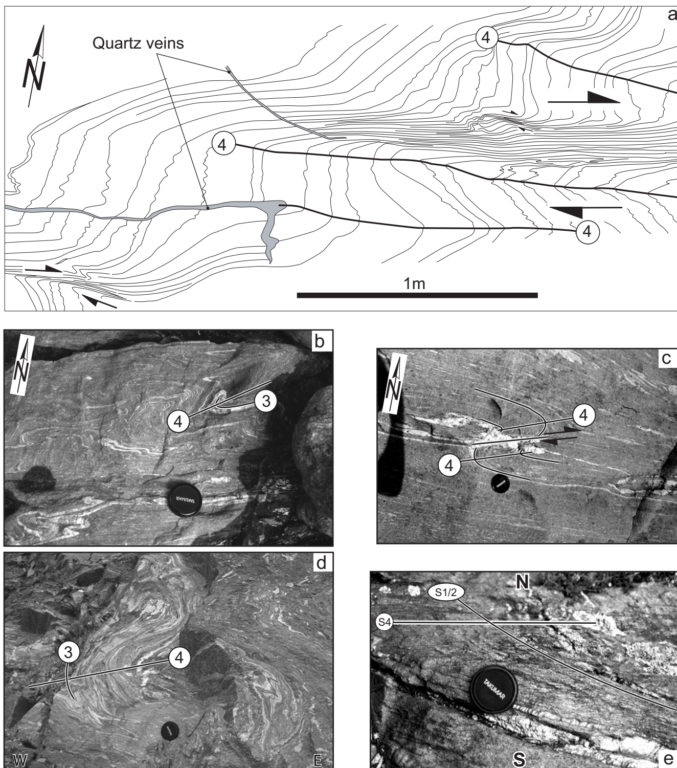
Fig. 8. D4 fold structures within paragneisses from the Camughera-Moncucco unit in Val Antrona. Figure 8a is from north of the axial plane of the Vanzone antiform; Figures 8b, c are from an outcrop situated south of the Vanzone axial plane; Figures 8d, e are situated south of Vanzone axial plane. Note the changing asymmetry of D4 folds across the hinge of the Vanzone antiform, while the sense of shear (Fig. 8a, c) remains the same.
