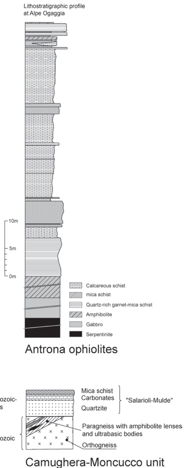
Fig. 3. Lithostratigraphic profile of the Antrona ophiolites taken at Alpe Ogaggia (see Fig. 2 for location and synthetic lithostratigraphic profile of the Camughera-Moncucco unit).
