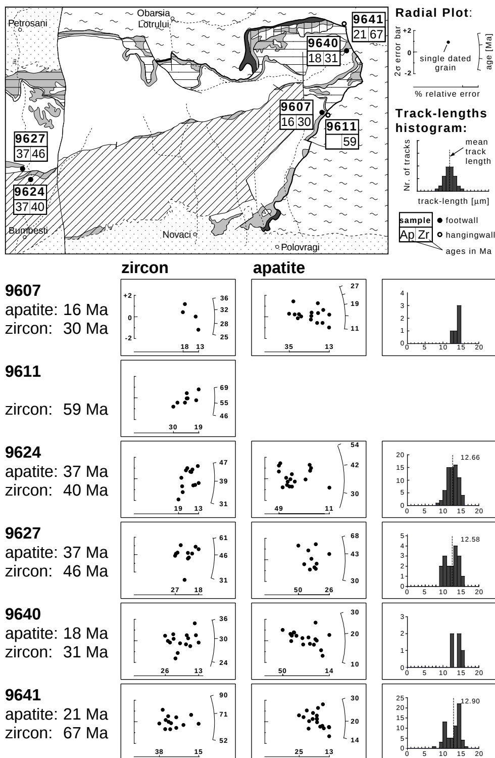
Fig. 8. Zircon and apatite fission-track ages, together with radial plots (Galbraith, 1990) for single grain age distributions and track lengths histograms for confined horizontal tracks in apatite. Sample localities are indicated in the tectonic map of the Parang mountains (cf. Fig. 3).
