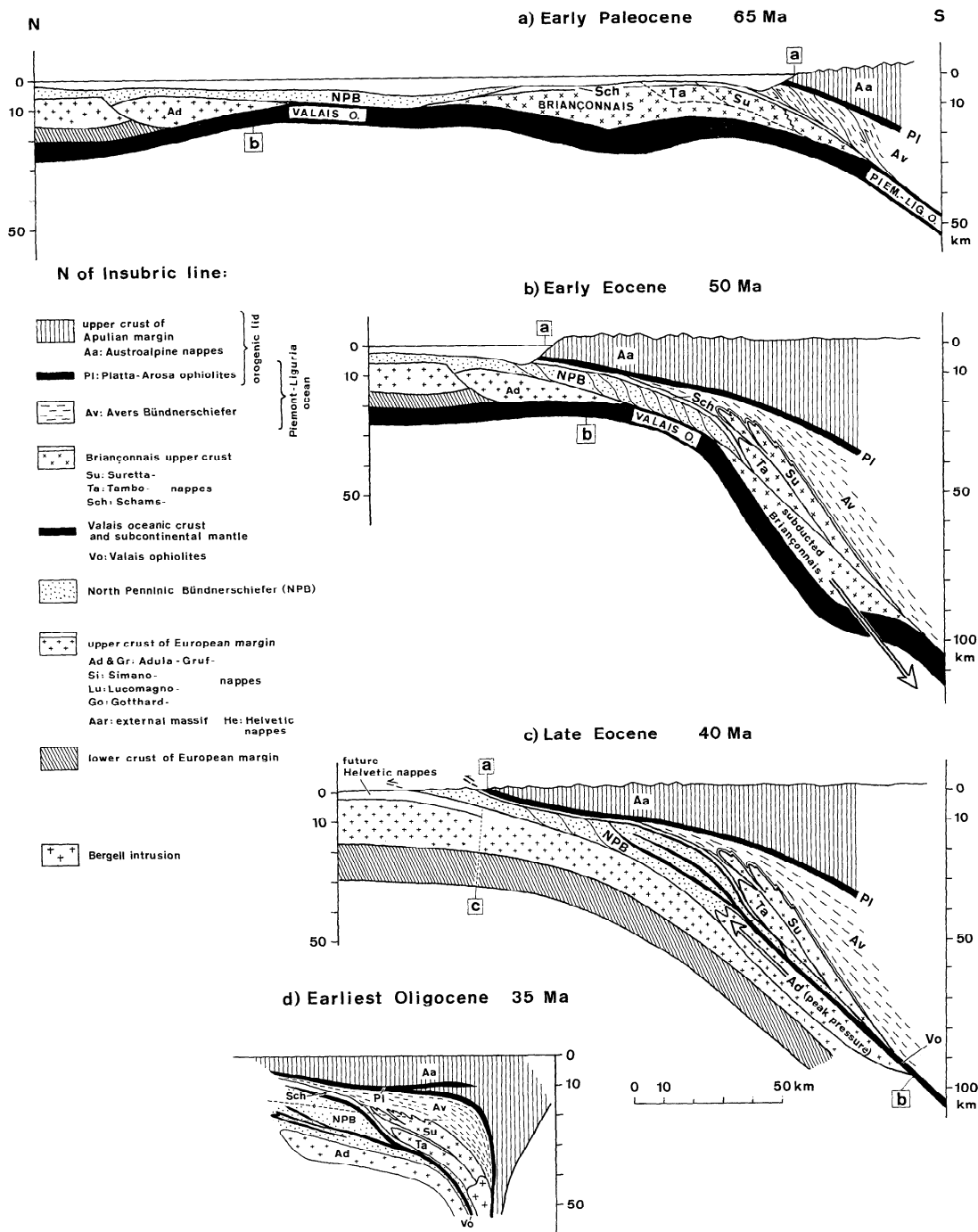
Figure 8. Scaled and area-balanced sketches of the kinematic evolution of the eastern Central Alps from (a-b) early Tertiary convergence and subduction to (c) collision and (d-g) postcollisional shortening.
