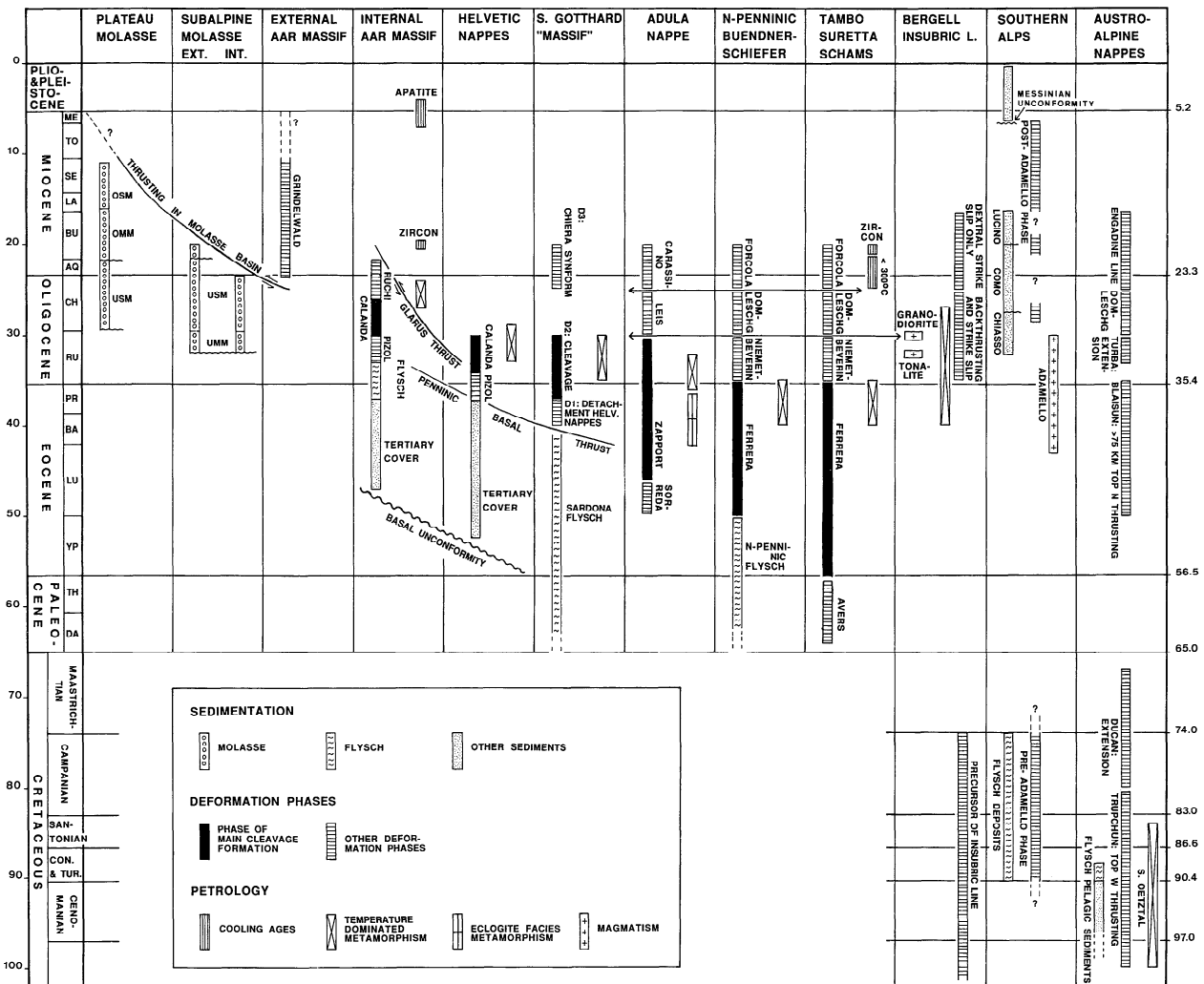
Figure 4. Correlation table showing an attempt to date deformation phases and metamorphism along the transect of Plate 1. Timescale is according to Harland et al. [1989]. The abbreviations UMM, USM, OMM, and OSM denote the Lower Marine Molasse, Lower Freshwater Molasse, Upper Marine Molasse, and Upper Freshwater Molasse, respectively. See text for further explanations. For an extensive discussion, see Schmid et al. [1996].
