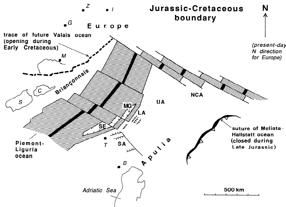
Figure 5. Paleogeographic reconstruction for the Jurassic-Cretaceous boundary, after Dercourt et al. [1986], Stampfli [1993], and Schmid et al. [1996], showing the oceanic suture of the former Meliata-Hallstatt Ocean, the Piemont-Liguria (South-Penninic) Ocean, and the trace along which the Valais (North-Penninic) Ocean will open. Abbreviations are SE, Sesia-Dentblanche extensional allochthon; MG, Magna extensional allochthon; SA, passive continental margin of Southern Alps; LA, Lower Austroalpine realm; UA, Upper Austroalpine realm; NCA, Northern Calcareous Alps. Geographical reference points are S, Sardinia; C, Corsica; M, Marseille; G, Geneva; Z, Zürich; I, Innsbruck; T, Torino; and B, Bologna.
