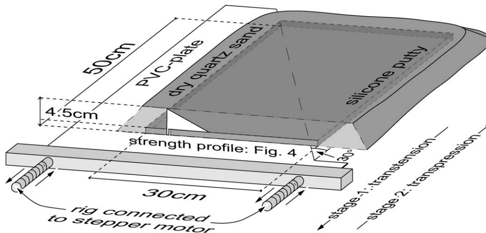
Fig. 5. Schematic block diagram of the experimental setup. A rectangular block of silicone putty ( 50 \times 30 \times 0.5 cm) is entirely covered by 4 cm of dry quartz sand. Deformation in the two-layer model is induced by a 1 mm thick, rigid basal PVC plate, which is driven by an electronically controlled stepper motor.
