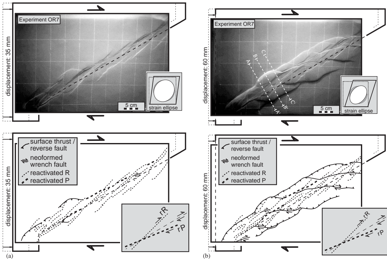
Fig. 11. Oblique rift model (transensional wrench faulting, experiment OR7), transpressively reactivated at a high displacement rate of 5 cm/h. Compare Fig. 6 for oblique rift stage before transpressional reactivation. rR = reactivated R-type fault, rP = reactivated P-type fault. (a) Deformation pattern after 35 mm of transpressive displacement. Illumination is from above. (b) Deformation pattern at the end of the experiment (after 60 mm of displacement). Illumination from top part of figure. Locations of cross-sections are indicated by dashed white lines.
