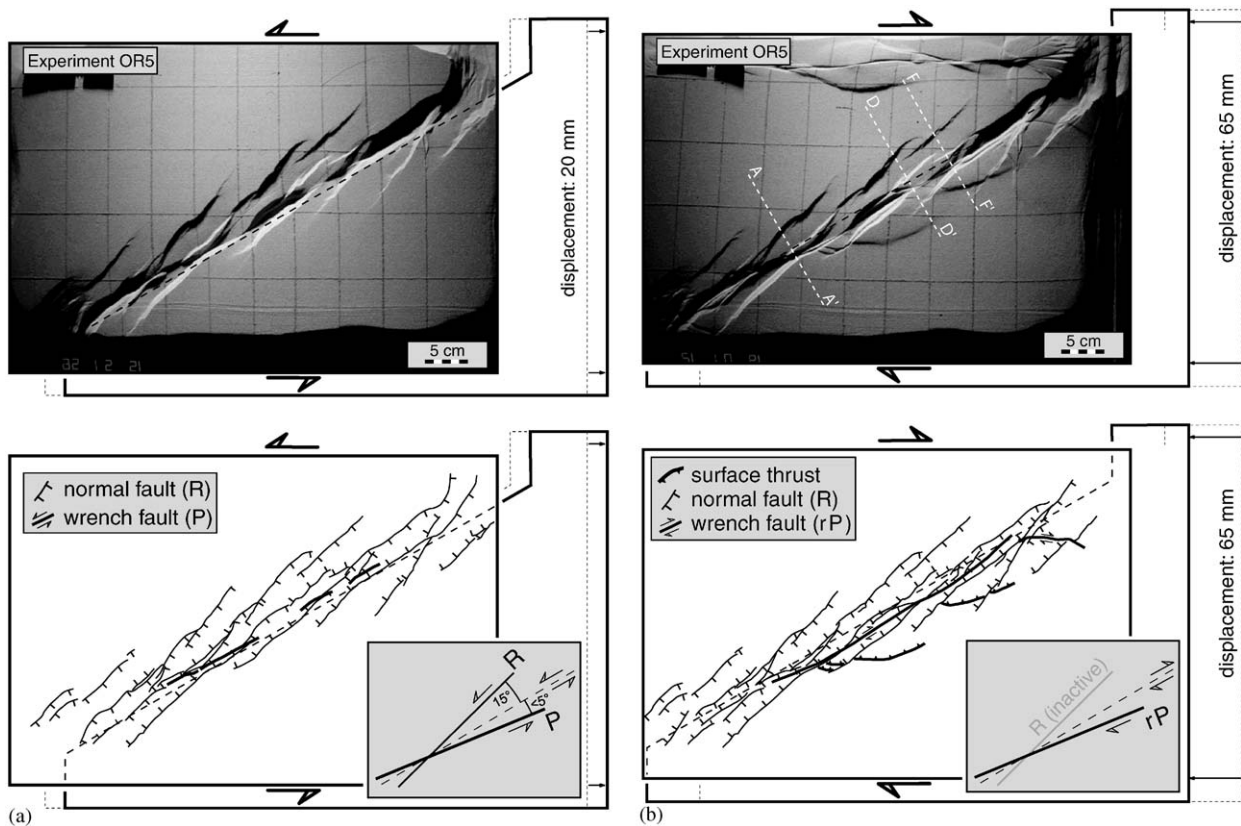
Fig. 9. (a) Fault patterns of an oblique rift model (transtensional wrench faulting, experiment OR5) after 20 mm of transtension. Illumination from top part of figure. Local depocenters are formed by linkage of R- and P-shears as well as by the corrugation of fault ends. (b) Fault pattern of the same experiment after subsequent transpressional reactivation at a low displacement rate of 2.6 cm/h and 65 mm displacement. No inversion of the graben occurred. Illumination is from above. Strike-slip fault in top-part of the picture represents boundary effect due to lateral confinement of the silicone putty, but did not affect structures evolving in central rift. Locations of cross-sections (Fig. 10) indicated. rP = reactivated P-type fault.
