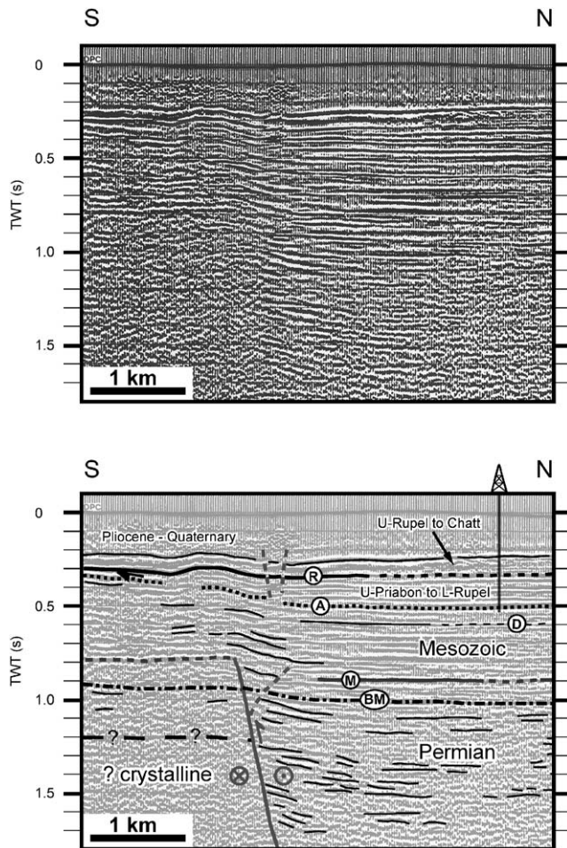
Fig. 3. N-S-trending reflection seismic line crossing a reactivated ENE-trending basement fault in the southernmost Upper Rhine Graben. For the location see Fig. 2. (a) un-migrated, stacked time section, b: interpreted section. BM=base Mesozoic, M=top Muschelkalk, D=top Dogger, A=top Malm, R=Upper Rupelian. During Eo- to Oligocene rifting, an extensional flexure has developed in the Mesozoic sediments above a north-dipping normal fault, delimiting a Permo-Carboniferous trough (note the differently reflective basement beneath the Mesozoic across the fault). Synrift sediments show a southward-tapering wedge and are of Upper Priabonian to Late Chattian age. Compressive/transpressive reactivation of the normal fault led to the inversion of the flexure, evidenced in the gently folded Upper Rupelian reflector (marked "R"). Seismic data courtesy of Shell International EP.
