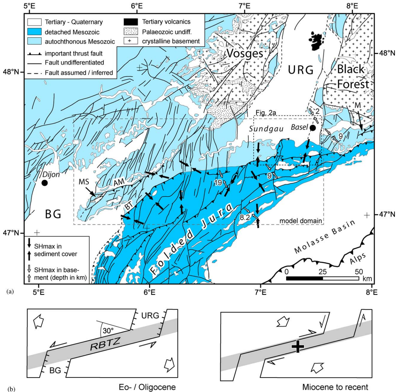
Fig. 1. (a) Geological overview of the western European Rhine-Bresse transfer zone (RBTZ), connecting the Bresse Graben (BG) and Upper Rhine Graben (URG). Maximum horizontal stress orientations in cover (black double arrows) and basement (white double arrows), derived from in-situ stress measurements and earthquake focal mechanisms (Becker, 2000; Reinecker et al., 2003; Häring, 2001) are shown. Note decoupled stresses between basement and cover particularly in the eastern Folded Jura. Large dashed rectangle depicts the modelled domain. AM = Avant-Mont thrust, BT = Besançon thrust, MS = Massif de la Serre, M = Mandach and Mettau thrusts. Small dashed rectangle indicates position of Fig. 2a. (b) Sketches of the kinematic framework of the RBTZ from Palaeogene to recent times. “+” indicates uplift (modified after Lacombe et al., 1993).
