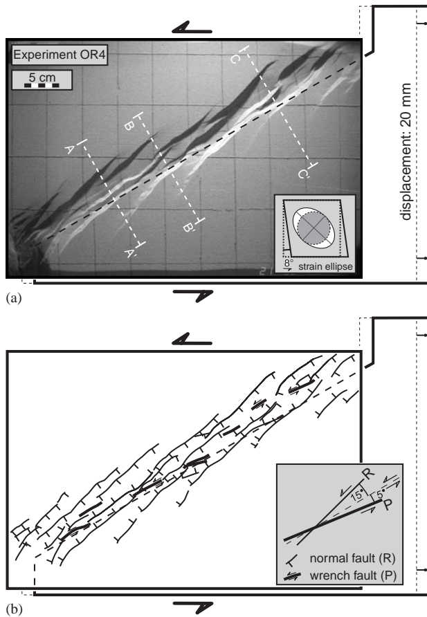
Fig. 7. Oblique rift model (transensional wrench faulting, experiment OR4). Illumination from top part of figure. (a) Fault pattern and representative strain ellipse after 20 mm transensional displacement. Locations of cross-sections (Fig. 8) are indicated. (b) Line drawing of the fault pattern. Note the switch in normal fault polarity with respect to the location of P-shears.
