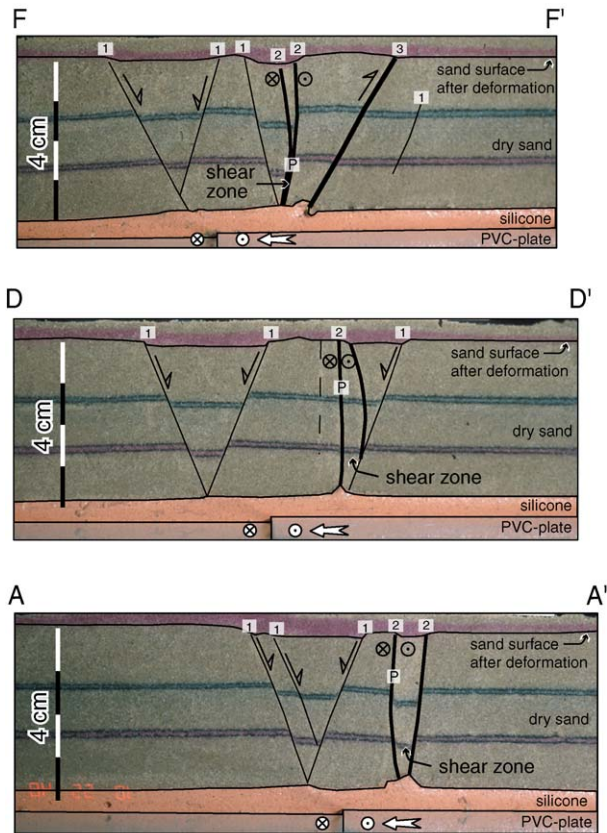
Fig. 10. Cross-sections through a transpressively reactivated oblique rift model (low displacement rate, experiment OR5). For locations see Fig. 9b. Numbers 1 to 3 indicate the nature of faults during transpressional reactivation. (1) not reactivated (R-type) faults, (2) reactivated (P-type) faults, (3) reverse faults formed during transpressional reactivation. Reactivated and neo-formed faults are drawn with thicker stroke. Note the slightly thickened silicone in the vicinity of the edge of the basal plate.
