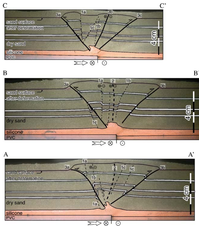
Fig. 12. Cross sections through a transpressively deformed oblique rift model (high displacement rate, experiment OR7). For locations see Fig. 11b. Numbers 1–3 indicate the nature of faults during transpressional reactivation. (1) reactivated R-type faults, (2) reactivated P-type faults, (3) neo-formed reverse faults. Lower case letters indicate relative sequence in which the individual faults appear in the section plane by along-strike propagation. Strokes and dashes correspond to Fig. 11.
