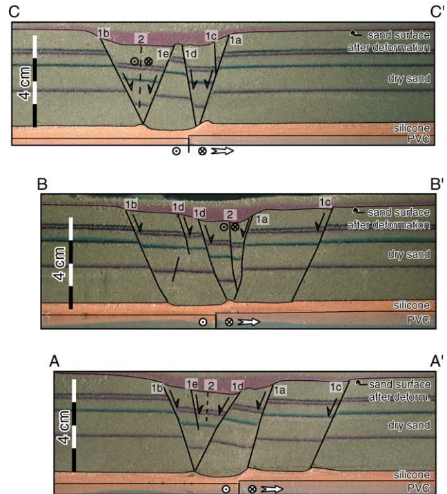
Fig. 8. Cross-sections across the oblique rift structure (experiment OR4) after 20 mm transension. For location of the sections see Fig. 7. Note the characteristic thinning or “necking” of the viscous base below the graben. Genetic chronology of faults is indicated by numbers 1 and 2. Lower case letters indicate relative chronology in which the individual faults appear in the section plane by along-strike propagation. First faults (1a, 1b) are synthetic R-type shears and form the external boundary faults of the graben. Along-strike propagation of these en-échelon aligned faults (labelled “1c”) causes widening of the rift. Younger R-type faults (1d, 1e) form in the interior part of the rift. Faults of generation 2 are P-type shears and form in the centre of the rift.
