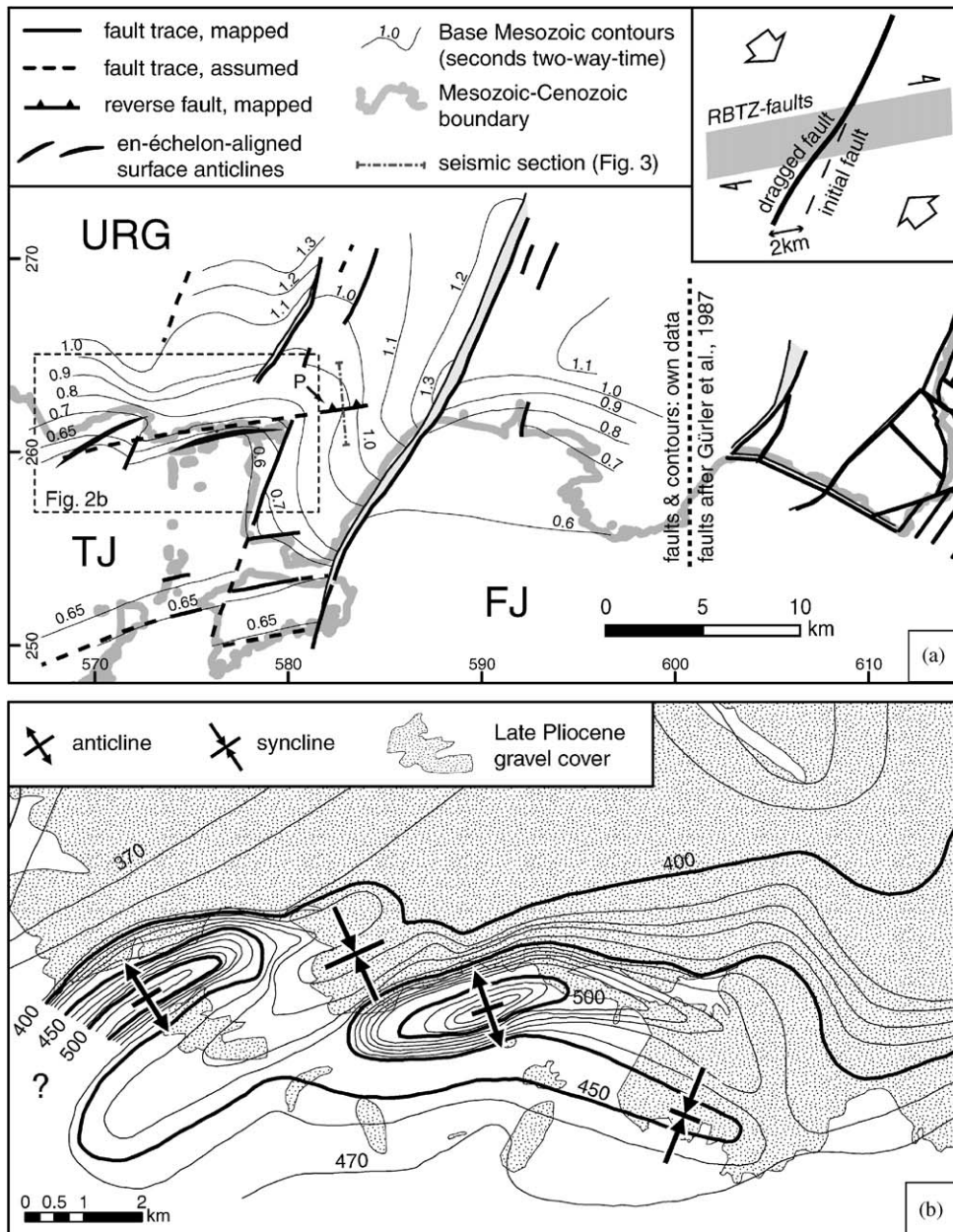
Fig. 2. (a) Close-up on a part of the southernmost Upper Rhine Graben (URG) and adjacent Jura Mountains, showing faults dissecting the Base Mesozoic (western part) and Top-Buntsandstein surfaces (eastern part of figure). Note the systematic dextral drag of N20°-trending faults along ENE-trending faults, which is interpreted as the result of dextral reactivation of ENE-trending faults in the Neogene (insert at top right). Numbers at edges refer to Swiss National grid. FJ = Folded Jura, TJ = Tabular Jura, P = Pfetterhouse reverse fault. (b) Contours of the base of Late Pliocene Sundgau gravels (in m above sea level; isohypse distance 10 m) in the area of en-échelon aligned surface anticlines, testifying to Post-Late Pliocene to recent shortening (after Giamboni et al., 2004).
