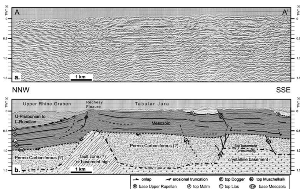
Fig. 5 NNW–SSE-trending reflection-seismic line crossing the E–W-trending extensional Réchény flexure at the URG–Jura boundary (data courtesy of Shell International EP). For location see Fig. 4. a un-migrated, stacked time section, b interpreted section
