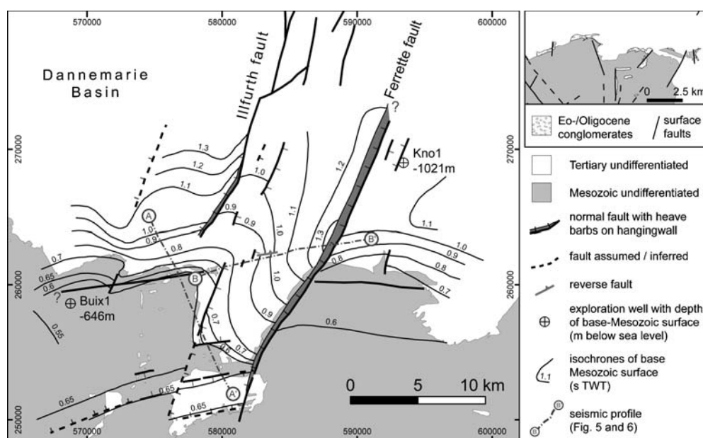
Fig. 4 Structural map of the base-Mesozoic surface in s TWT and dissecting faults. The reference datum is at 500 m above sea level. Numbers on map margin refer to Swiss National coordinates. Top right inset : distribution of Eo-/Oligocene conglomerates along the en-échelon flexures
