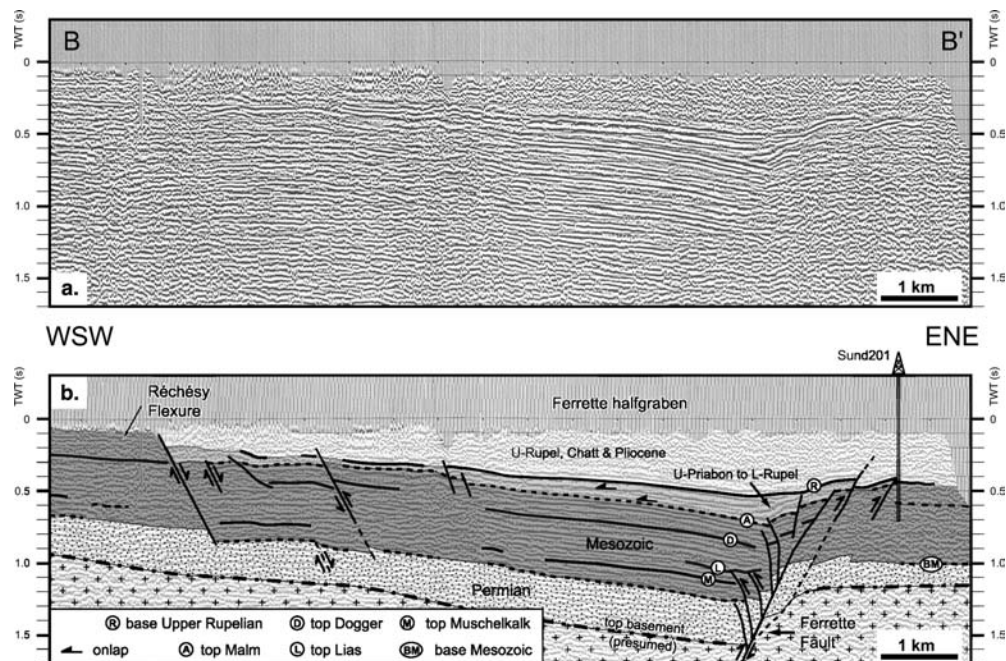
Fig. 6 WSW–ENE-trending reflection-seismic line across the NNE-trending Ferrette half-graben bounded by URG-parallel normal faults (data courtesy of Shell International EP). For location see Fig. 4. a un-migrated, stacked time section, b interpreted section
